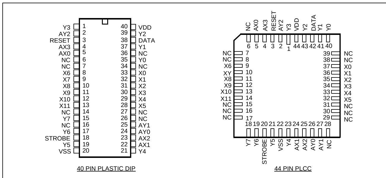
Figure 2 - Pin Connections
